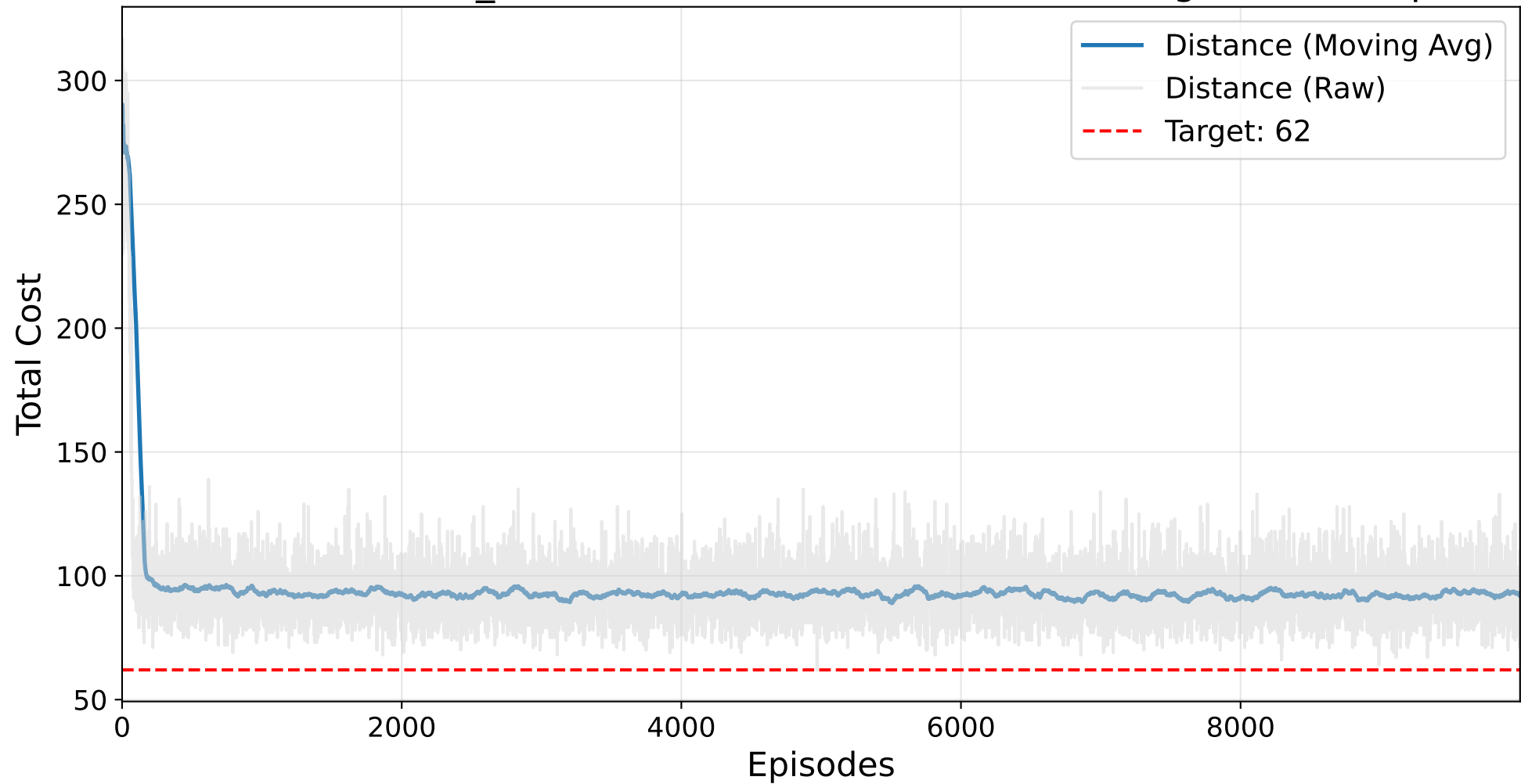
Final RANDOM_SEARCH Masked AutoRL-SOP Training - ESC63.sop
